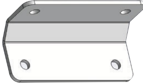
CORNER JOINING PART DETAIL-B
