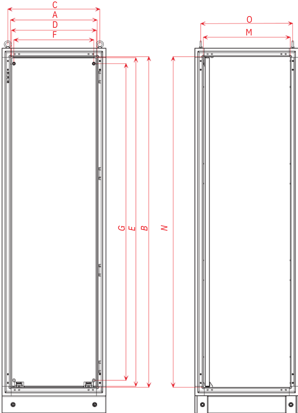
FRONT VIEW (WITHOUT FRONT DOOR)
