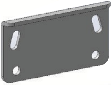
SIDE JOINING PART DETAIL-A
