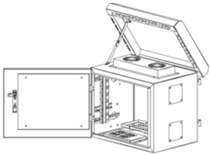
FRONT DOOR AND TOP COVER OPEN, ISOMETRIC VIEW
