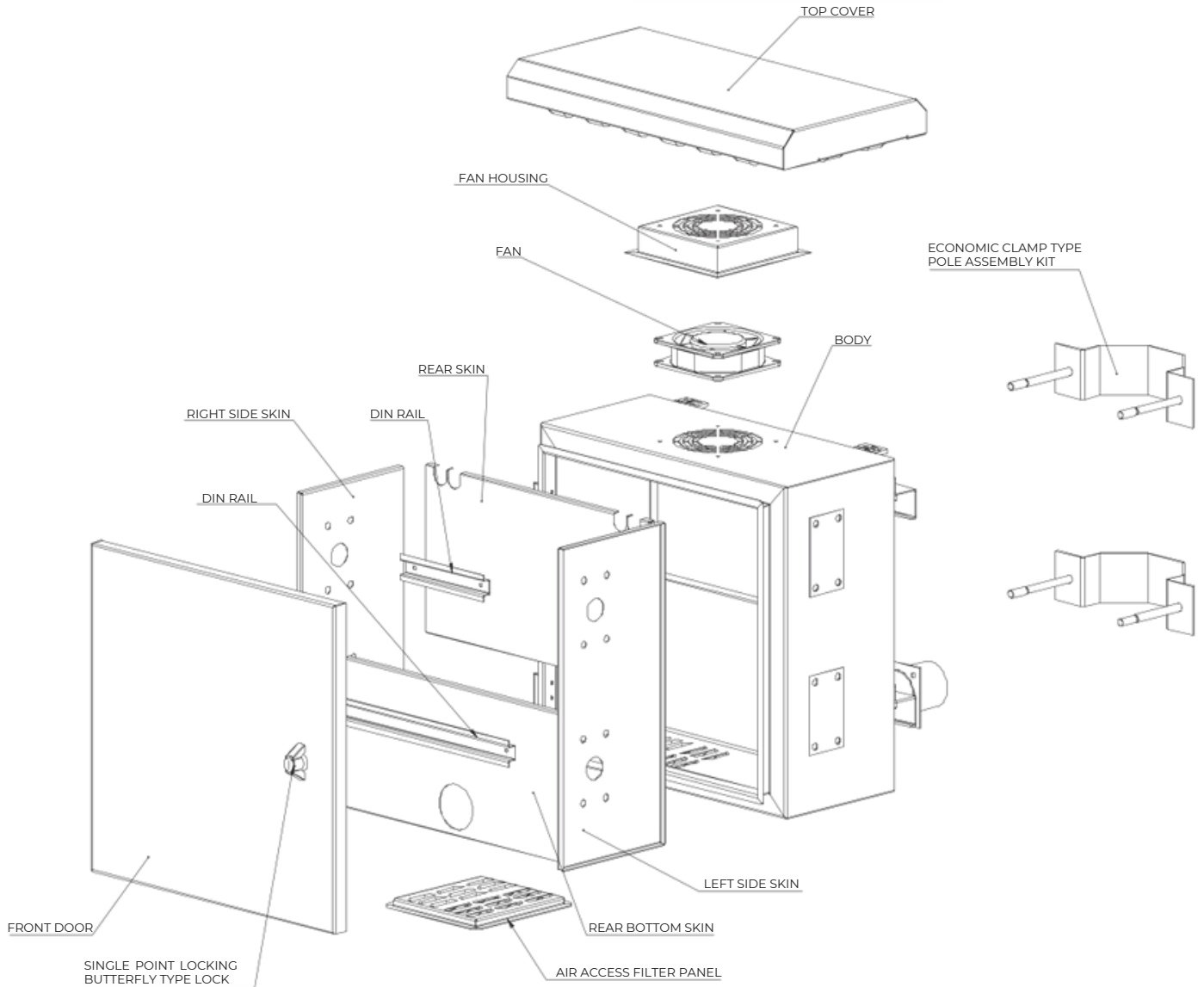
EXPLODED VIEW
