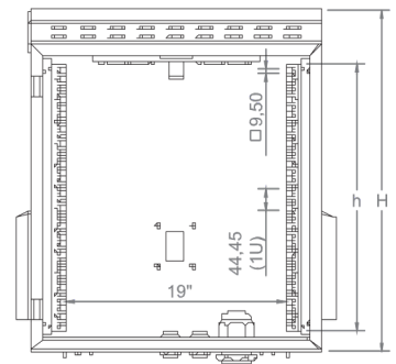
Inside view
