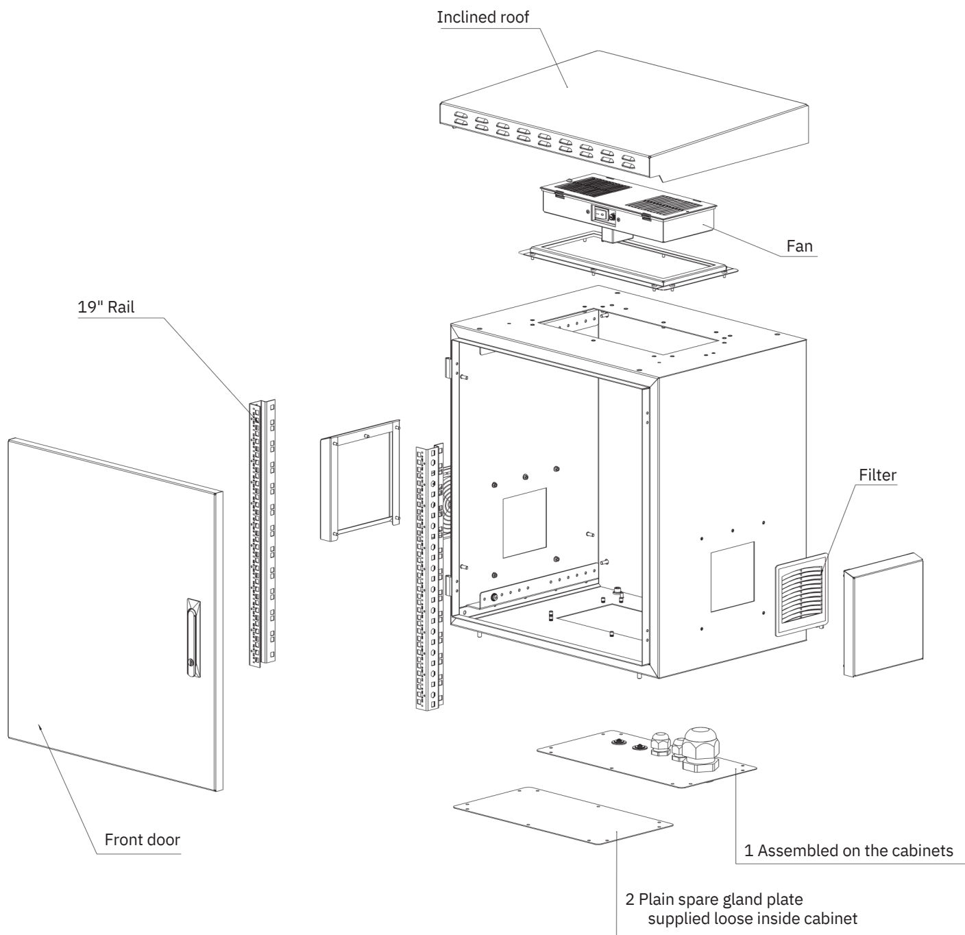
Exploded view
